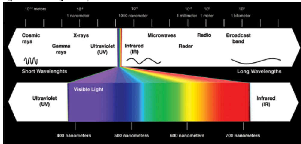
Fig 1. Electromagnetic Spectrum
