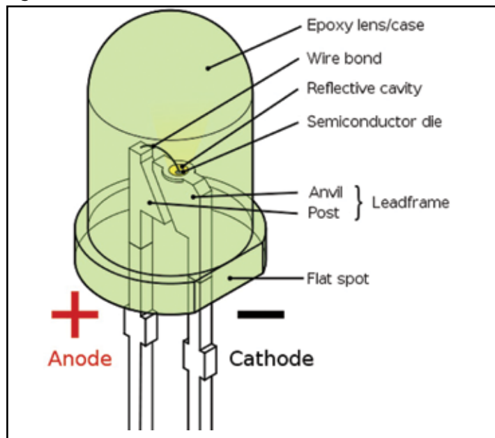
Fig 2. LED schematic
